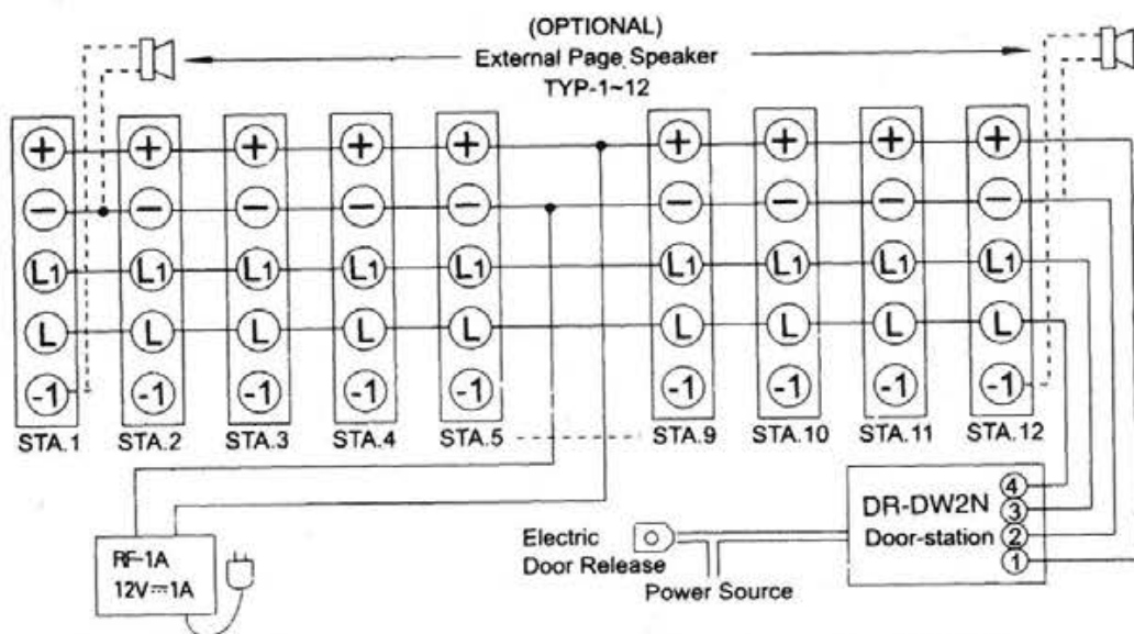
Figure-5 TP-nRC and DR-DW2N Connection Diagram
